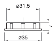
162 E 14 Schraubring H = 7mm, DM 33
